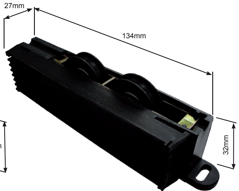
DR401 - Double
