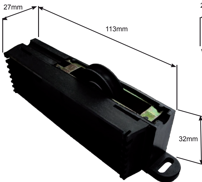
DR400 - Single
